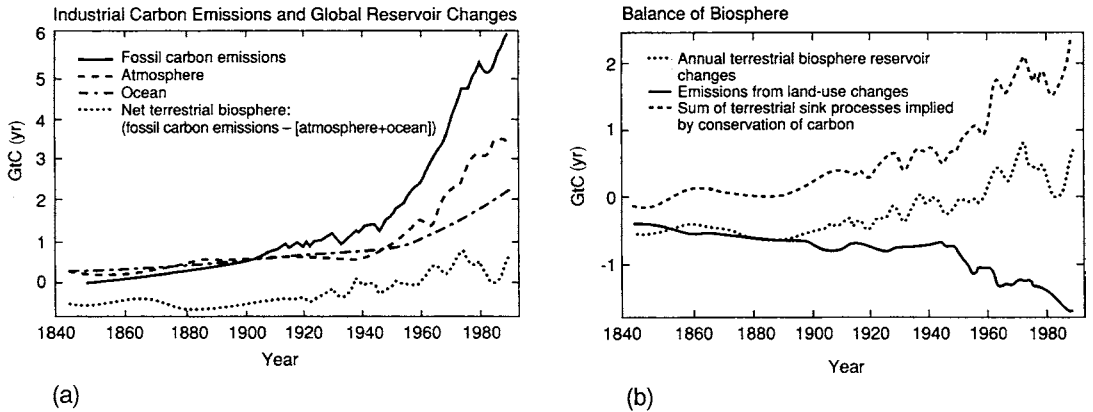
Figure 3.3 (a) Fossil carbon emissions (based on statistics of fossil fuel and cement production) and estimates of global reservoir changes: atmosphere (deduced from direct observations and ice core measurements), ocean (calculated with the Geophysical Fluid Dynamics Laboratory (GFDL), University of Princeton, ocean carbon model) and net terrestrial biosphere (calculated as remaining imbalance) from 1840 to 1990. The calculation implies that the terrestrial biosphere was a net source to the atmosphere prior to 1940 (negative values) and has been a net sink since about 1960. (b) Estimates of contributions to the carbon balance of the terrestrial biosphere. The curve showing the terrestrial reservoir changes is taken from (a). Emissions from land-use changes (including tropical deforestation) are plotted negatively because they represent a loss of biospheric carbon. These estimates are subject to large uncertainties (see uncertainty estimates in Table 3.1).
