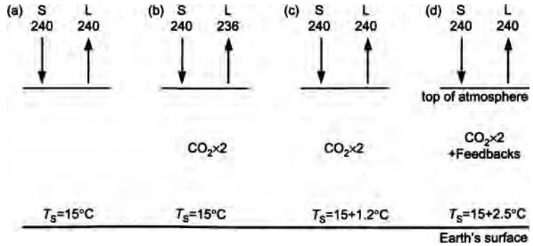
Figure 2.8 Illustrating the enhanced greenhouse gas effect. Under natural conditions (a) the net solar radiation coming in ( S = 240 watts per square metre) is balanced by thermal radiation (L) leaving the top of the atmosphere; average surface temperature ( T_s ) is 15^\circ\text{C} . If the carbon dioxide concentration is suddenly doubled (b), L is decreased by 4 watts per square metre. Balance is restored if nothing else changes (c) apart from the temperature of the surface and lower atmosphere, which rises by 1.2^\circ\text{C} . If feedbacks are also taken into account (d), the average temperature of the surface rises by about 2.5^\circ\text{C} .
