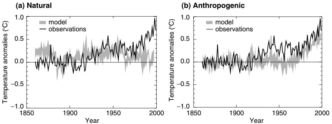
Figure 5.22 Annual global mean surface temperatures simulated by a climate model compared with observations for the period 1860–2000. The simulations in (a) were done with only natural forcings – solar variation and volcanic activity; in (b) with only anthropogenic forcings – greenhouse gases and sulphate aerosols; and in (c) with both natural and anthropogenic forcings combined. The simulations are shown in a band that covers the results from four runs with the same model and therefore illustrates the range of natural variability within the model.
