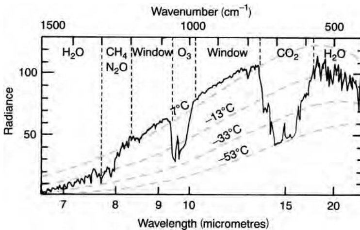
Figure 2.4 Thermal radiation in the infrared region (the visible part of the spectrum is between about 0.4 and 0.7 μm) emitted from the Earth’s surface and atmosphere as observed over the Mediterranean Sea from a satellite instrument orbiting above the atmosphere, showing parts of the spectrum where different gases contribute to the radiation. Between the wavelengths of about 8 and 14 μm, apart from the ozone band, the atmosphere, in the absence of clouds, is substantially transparent; this is part of the spectrum called a ‘window’ region. Superimposed on the spectrum are curves of radiation from a black body at 7 °C, –13 °C, –33 °C and –53 °C. The units of radiance are watts per square metre per steradian per wavenumber.
