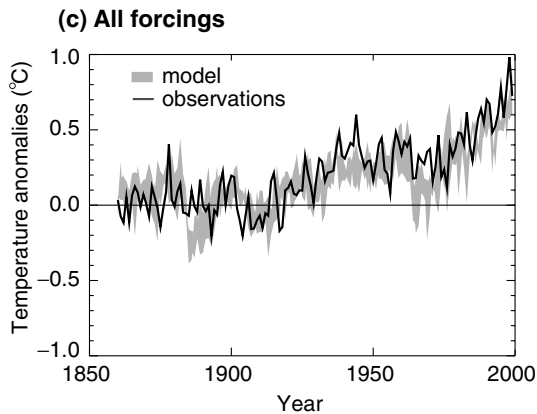
Figure 5.22 Annual global mean surface temperatures simulated by a climate model compared with observations for the period 1860–2000. The simulations in (a) were done with only natural forcings – solar variation and volcanic activity; in (b) with only anthropogenic forcings – greenhouse gases and sulphate aerosols; and in (c) with both natural and anthropogenic forcings combined. The simulations are shown in a band that covers the results from four runs with the same model and therefore illustrates the range of natural variability within the model.
